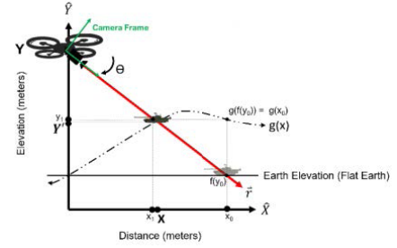
Fig 1. Shrike photogrammetric MGRS estimation example. Accurate estimates require a digital terrain and elevation dataset and some iterative algorithm.
