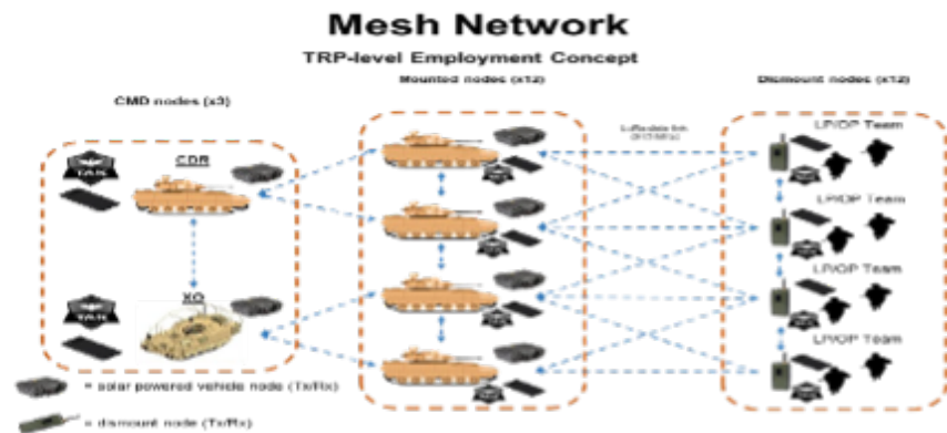
Fig 1. Troop-Level Mesh Network
