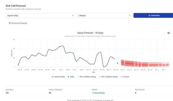
Fig 2. Sick Call Forecasting Module (forecast injuries).
