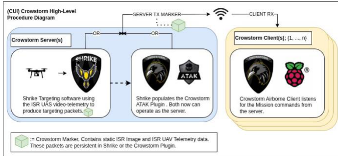
Fig 2. Crowstorm High-Level Diagram. The flow is UAS-Shrike-Crowstorm-engagement
