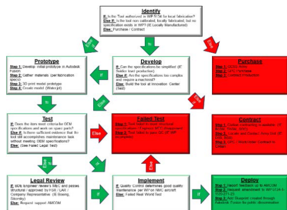
Fig 1. Fabrication Process
